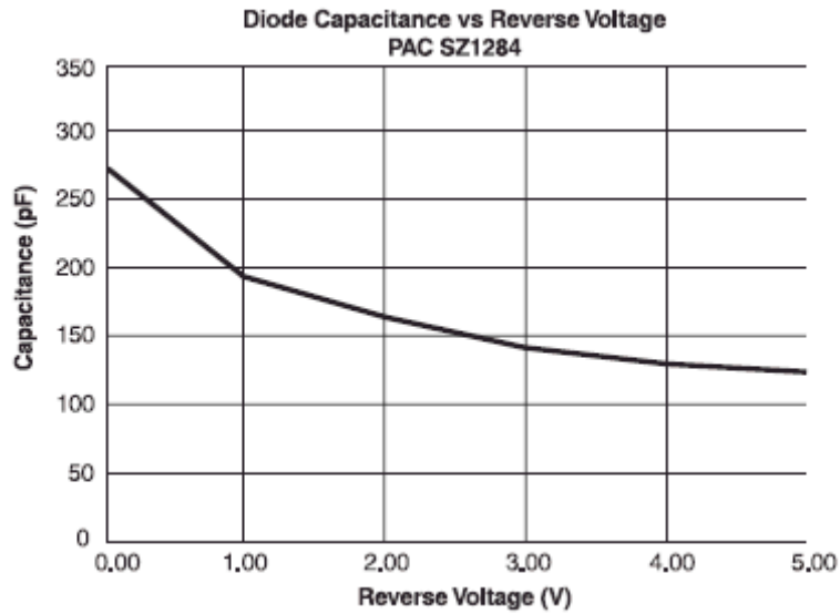
Figure 1. Diode Capacitance vs. Reverse Voltage
