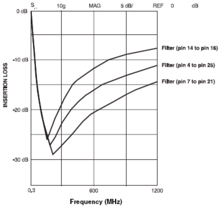
Figure 2. Typical Filter Insertion Loss
