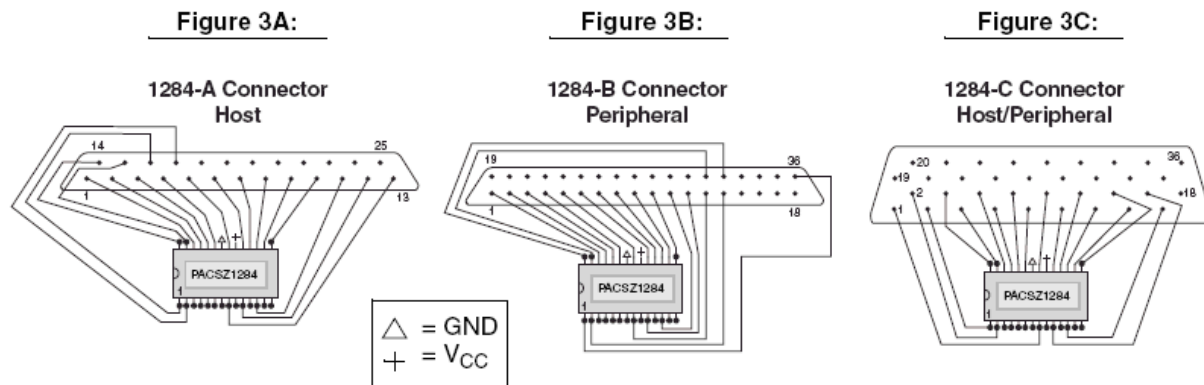
Figure 3. Example Connections of IEEE 1284 Connectors with PACSZ1284
